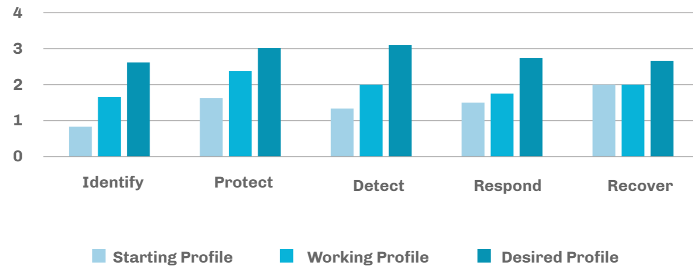
NIST Cyber Security Framework - Assessment Scoring
